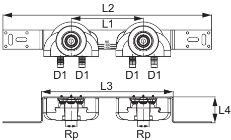
TECEflex assembly unit with wall disks made of silicone bronze and sound insulation boxes
