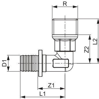
TECEflex male elbow
